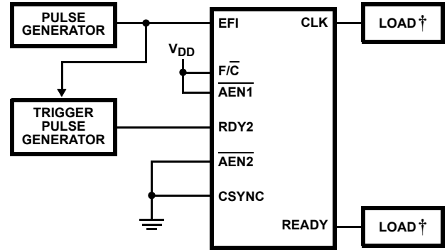
FIGURE 15. READY TO CLOCK (USING EFI)
